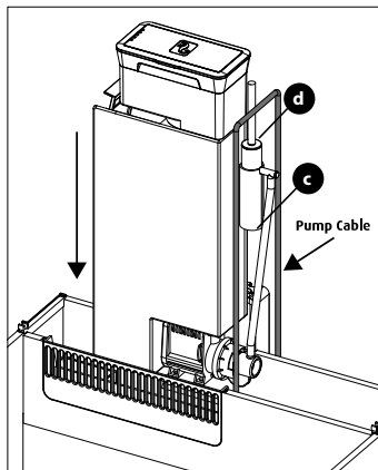
NANO skimmer
